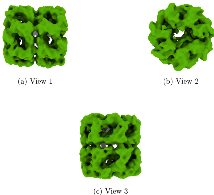
Figure 4: Isosurface at threshold=0.079700. Views generated by ChimeraX at a the following X, Y, Z angles: View 1 (0, -90, -90), View 2 (-90, 0, -90), View 3 (0, 0, 0).
