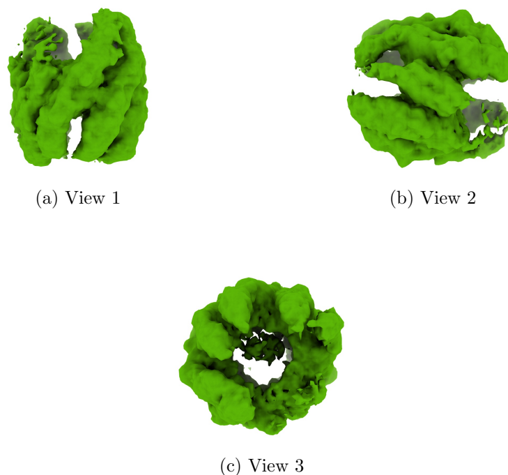
Figure 4: Isosurface at threshold=0.072000. Views generated by ChimeraX at the following X, Y, Z angles: View 1 (0, -90, -90), View 2 (-90, 0, -90), View 3 (0, 0, 0).
