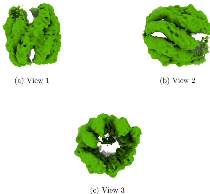
Figure 4: Isosurface at threshold=0.058500. Views generated by ChimeraX at a the following X, Y, Z angles: View 1 (0, -90, -90), View 2 (-90, 0, -90), View 3 (0, 0, 0).
