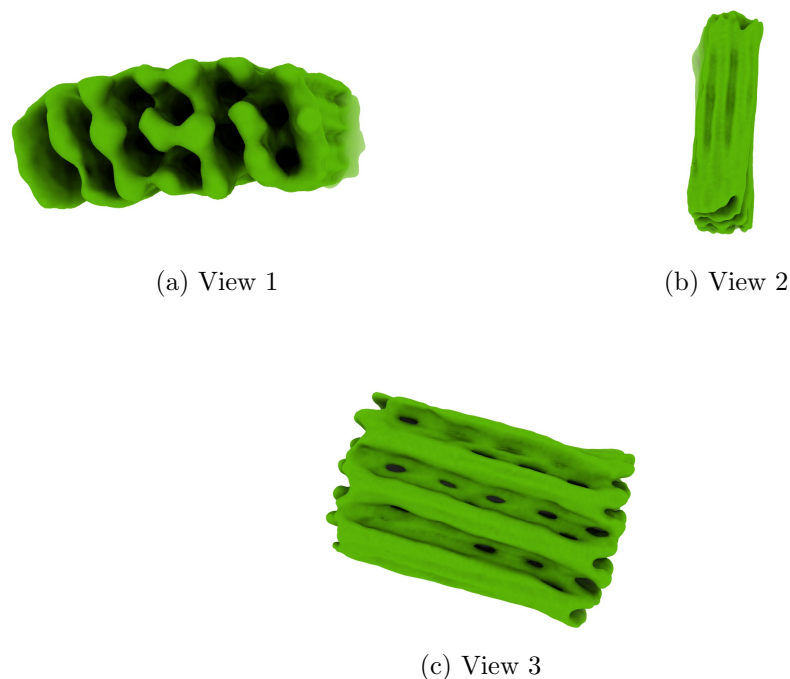
Figure 4: Isosurface at threshold=0.079000. Views generated by ChimeraX at a the following X, Y, Z angles: View 1 (0, -90, -90), View 2 (-90, 0, -90), View 3 (0, 0, 0).
