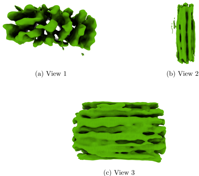
Figure 4: Isosurface at threshold=0.059000. Views generated by ChimeraX at a the following X, Y, Z angles: View 1 (0, -90, -90), View 2 (-90, 0, -90), View 3 (0, 0, 0).
