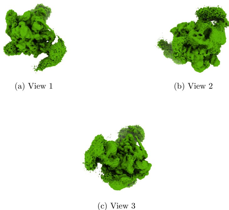
Figure 4: Isosurface at threshold=0.005760. Views generated by ChimeraX at a the following X, Y, Z angles: View 1 (0, -90, -90), View 2 (-90, 0, -90), View 3 (0, 0, 0).
