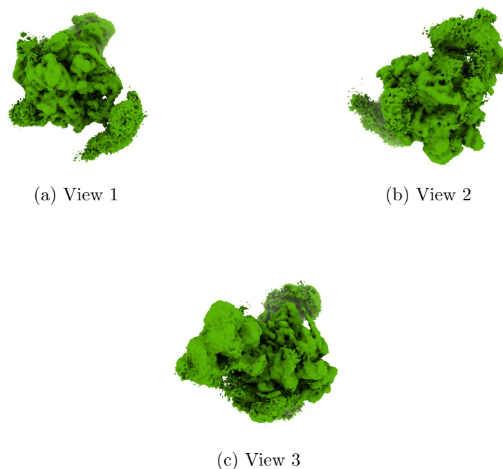
Figure 4: Isosurface at threshold=0.006020. Views generated by ChimeraX at a the following X, Y, Z angles: View 1 (0, -90, -90), View 2 (-90, 0, -90), View 3 (0, 0, 0).
