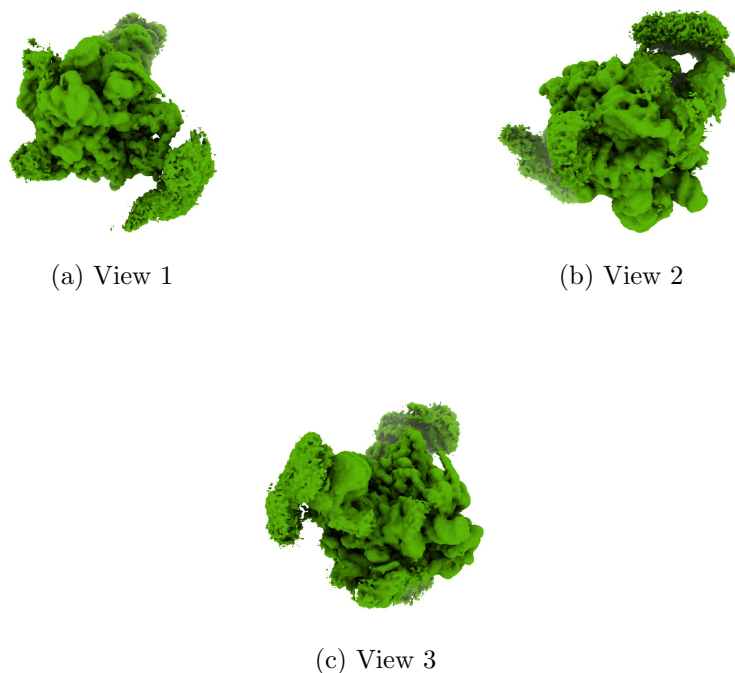
Figure 4: Isosurface at threshold=0.006200. Views generated by ChimeraX at a the following X, Y, Z angles: View 1 (0, -90, -90), View 2 (-90, 0, -90), View 3 (0, 0, 0).
