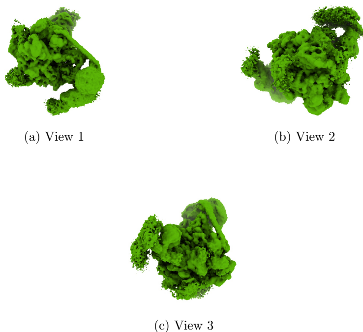
Figure 4: Isosurface at threshold=0.006670. Views generated by ChimeraX at a the following X, Y, Z angles: View 1 (0, -90, -90), View 2 (-90, 0, -90), View 3 (0, 0, 0).
