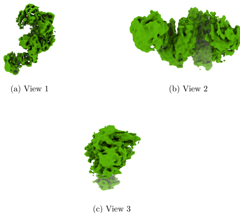
Figure 4: Isosurface at threshold=0.022100. Views generated by ChimeraX at a the following X, Y, Z angles: View 1 (0, -90, -90), View 2 (-90, 0, -90), View 3 (0, 0, 0).
