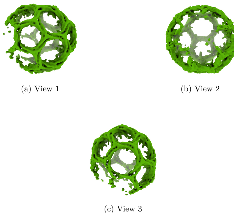
Figure 4: Isosurface at threshold=0.035800. Views generated by ChimeraX at a the following X, Y, Z angles: View 1 (0, -90, -90), View 2 (-90, 0, -90), View 3 (0, 0, 0).
