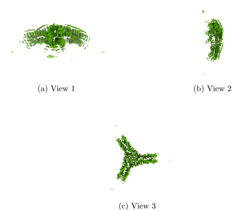
Figure 4: Isosurface at threshold=0.152000. Views generated by ChimeraX at a the following X, Y, Z angles: View 1 (0, -90, -90), View 2 (-90, 0, -90), View 3 (0, 0, 0).
