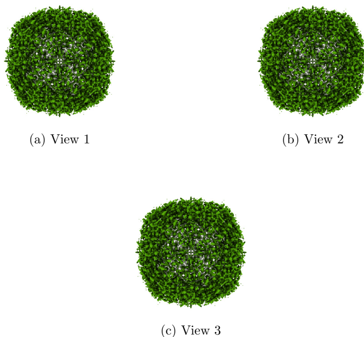
Figure 4: Isosurface at threshold=0.035000. Views generated by ChimeraX at the following X, Y, Z angles: View 1 (0, -90, -90), View 2 (-90, 0, -90), View 3 (0, 0, 0).
