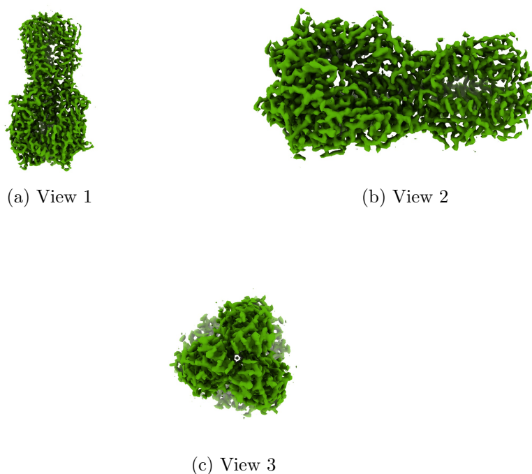
Figure 4: Isosurface at threshold=0.078000. Views generated by ChimeraX at a the following X, Y, Z angles: View 1 (0, -90, -90), View 2 (-90, 0, -90), View 3 (0, 0, 0).
