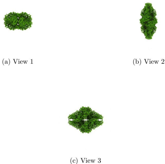
Figure 4: Isosurface at threshold=0.021000. Views generated by ChimeraX at a the following X, Y, Z angles: View 1 (0, -90, -90), View 2 (-90, 0, -90), View 3 (0, 0, 0).
