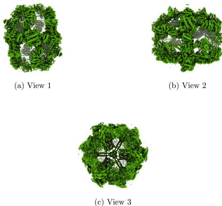
Figure 4: Isosurface at threshold=0.041900. Views generated by ChimeraX at a the following X, Y, Z angles: View 1 (0, -90, -90), View 2 (-90, 0, -90), View 3 (0, 0, 0).
