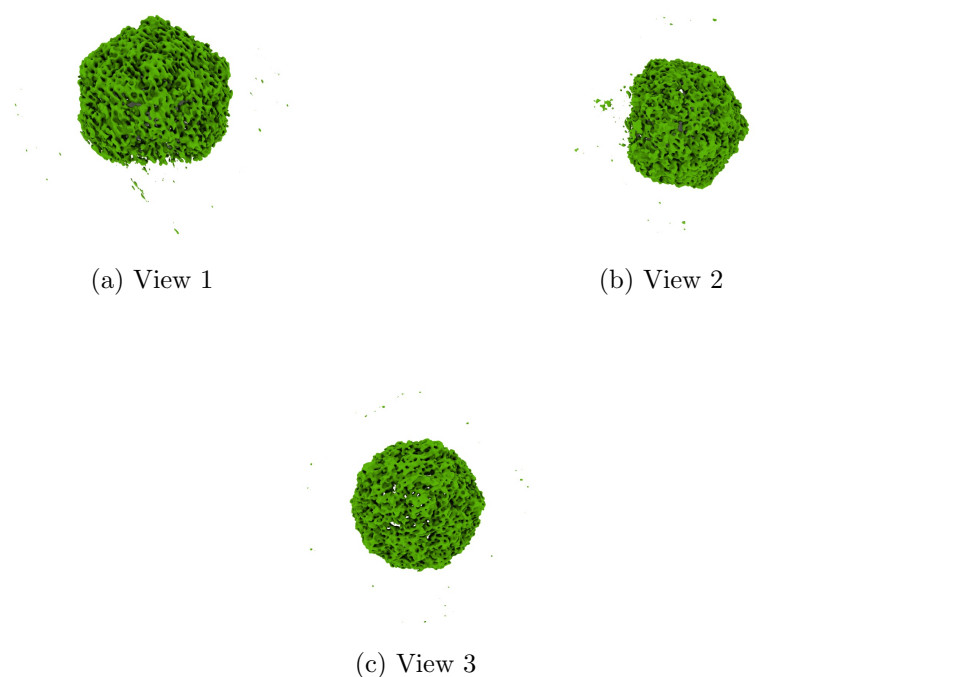
Figure 4: Isosurface at threshold=0.045000. Views generated by ChimeraX at a the following X, Y, Z angles: View 1 (0, -90, -90), View 2 (-90, 0, -90), View 3 (0, 0, 0).
