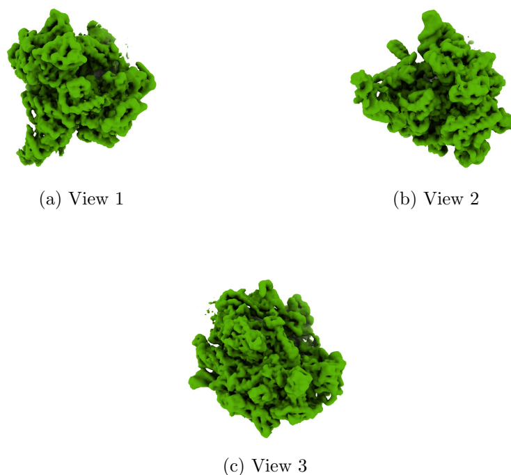
Figure 4: Isosurface at threshold=0.008710. Views generated by ChimeraX at a the following X, Y, Z angles: View 1 (0, -90, -90), View 2 (-90, 0, -90), View 3 (0, 0, 0).
