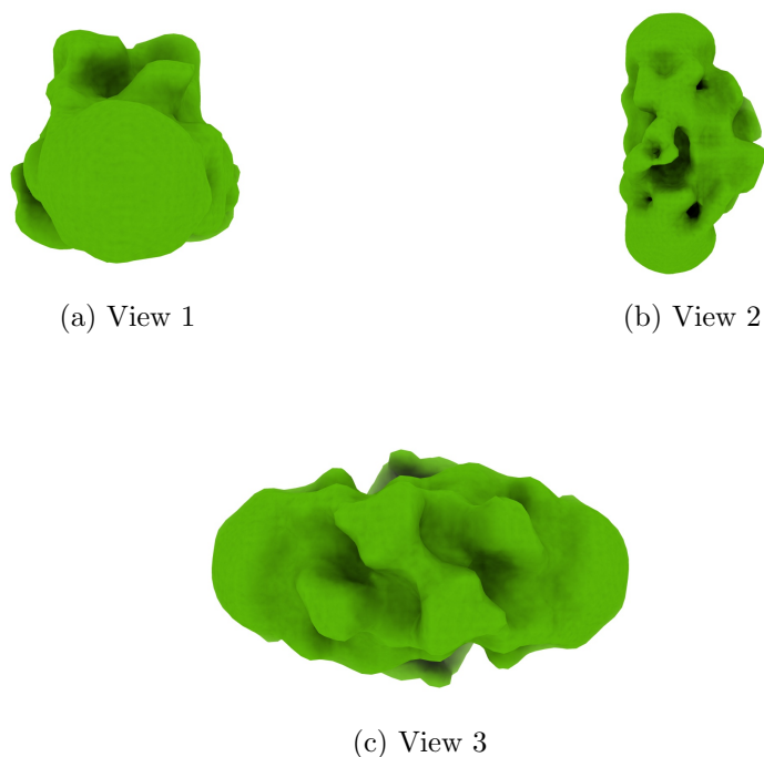
Figure 4: Isosurface at threshold=0.094000. Views generated by ChimeraX at a the following X, Y, Z angles: View 1 (0, -90, -90), View 2 (-90, 0, -90), View 3 (0, 0, 0).
