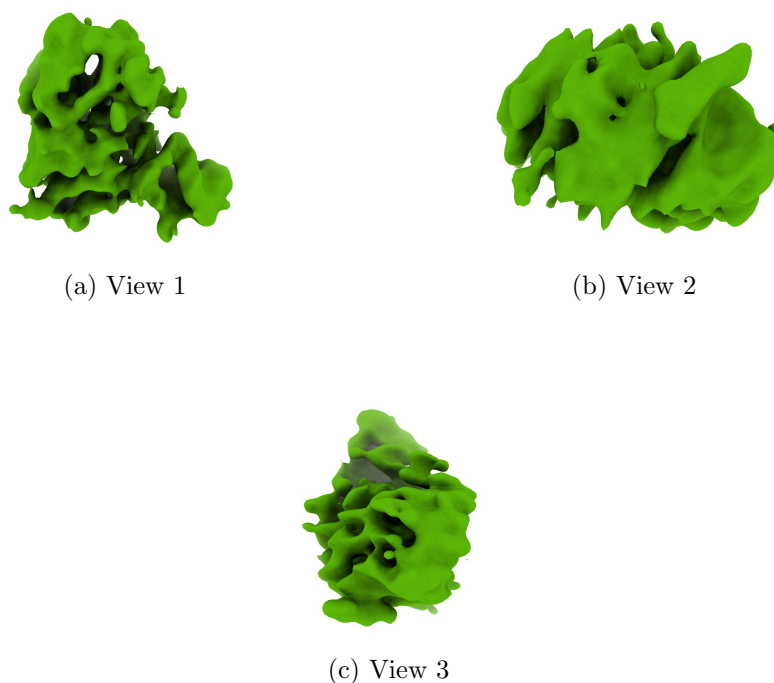
Figure 4: Isosurface at threshold=0.025000. Views generated by ChimeraX at a the following X, Y, Z angles: View 1 (0, -90, -90), View 2 (-90, 0, -90), View 3 (0, 0, 0).
