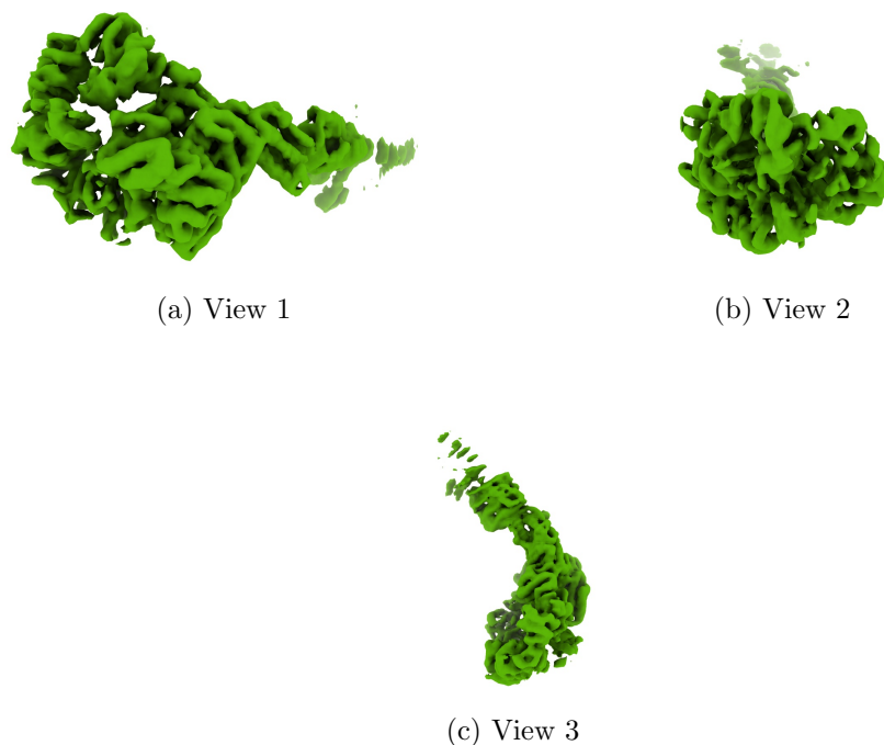
Figure 4: Isosurface at threshold=0.010600. Views generated by ChimeraX at a the following X, Y, Z angles: View 1 (0, -90, -90), View 2 (-90, 0, -90), View 3 (0, 0, 0).
