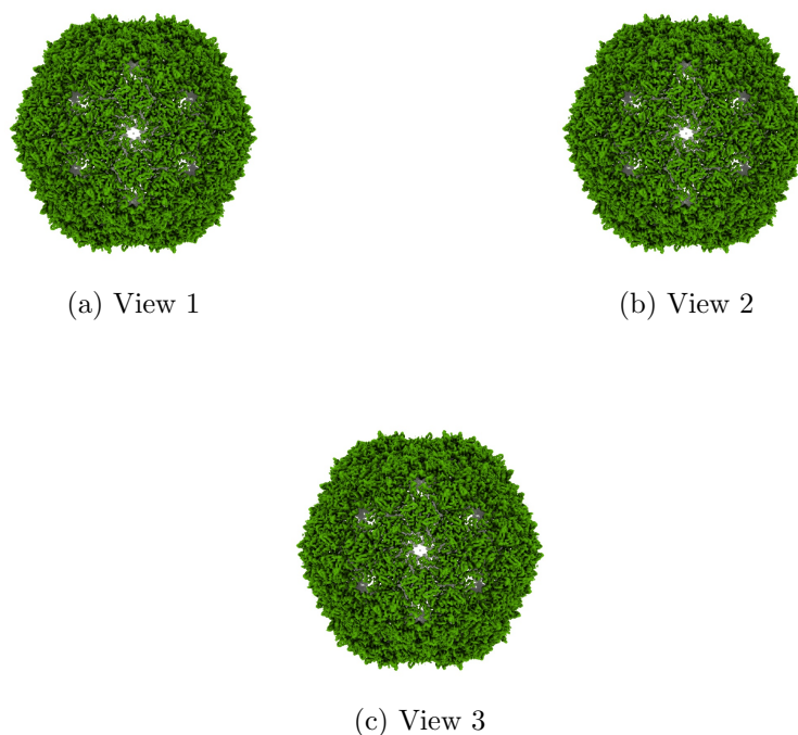
Figure 4: Isosurface at threshold=0.498000. Views generated by ChimeraX at a the following X, Y, Z angles: View 1 (0, -90, -90), View 2 (-90, 0, -90), View 3 (0, 0, 0).
