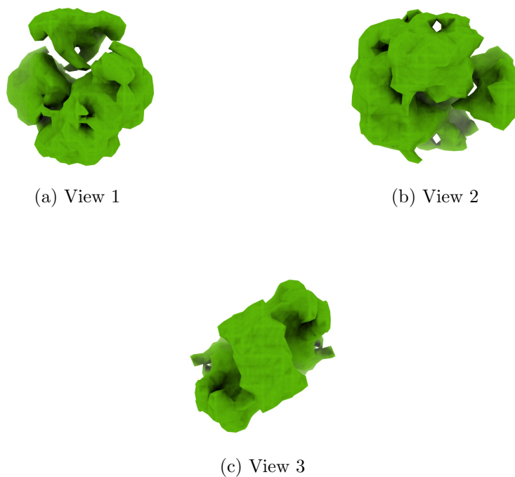
Figure 4: Isosurface at threshold=0.569000. Views generated by ChimeraX at a the following X, Y, Z angles: View 1 (0, -90, -90), View 2 (-90, 0, -90), View 3 (0, 0, 0).
