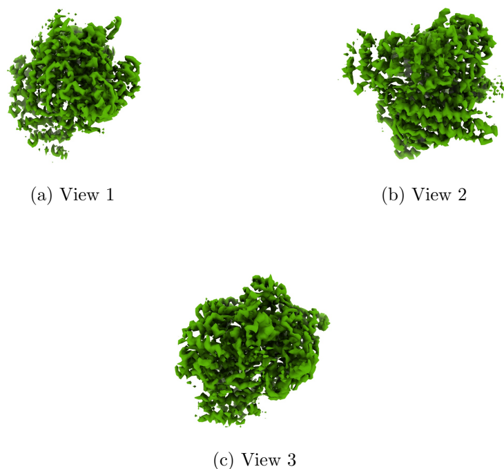
Figure 4: Isosurface at threshold=0.040000. Views generated by ChimeraX at a the following X, Y, Z angles: View 1 (0, -90, -90), View 2 (-90, 0, -90), View 3 (0, 0, 0).
