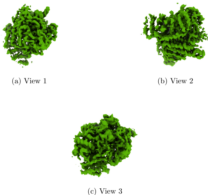
Figure 4: Isosurface at threshold=0.012700. Views generated by ChimeraX at a the following X, Y, Z angles: View 1 (0, -90, -90), View 2 (-90, 0, -90), View 3 (0, 0, 0).
