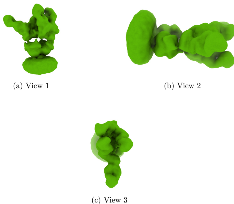
Figure 4: Isosurface at threshold=0.011800. Views generated by ChimeraX at a the following X, Y, Z angles: View 1 (0, -90, -90), View 2 (-90, 0, -90), View 3 (0, 0, 0).
