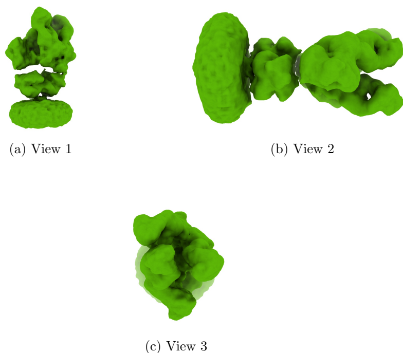
Figure 4: Isosurface at threshold=0.013700. Views generated by ChimeraX at a the following X, Y, Z angles: View 1 (0, -90, -90), View 2 (-90, 0, -90), View 3 (0, 0, 0).
