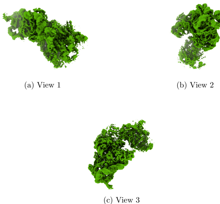
Figure 4: Isosurface at threshold=0.071800. Views generated by ChimeraX at a the following X, Y, Z angles: View 1 (0, -90, -90), View 2 (-90, 0, -90), View 3 (0, 0, 0).
