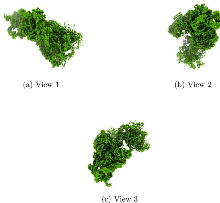
Figure 4: Isosurface at threshold=0.090100. Views generated by ChimeraX at a the following X, Y, Z angles: View 1 (0, -90, -90), View 2 (-90, 0, -90), View 3 (0, 0, 0).
