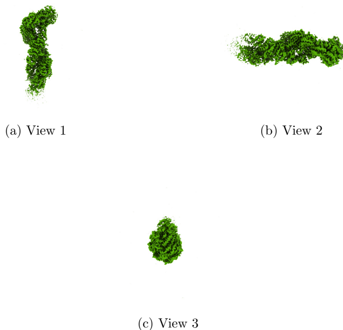
Figure 4: Isosurface at threshold=0.750000. Views generated by ChimeraX at a the following X, Y, Z angles: View 1 (0, -90, -90), View 2 (-90, 0, -90), View 3 (0, 0, 0).
