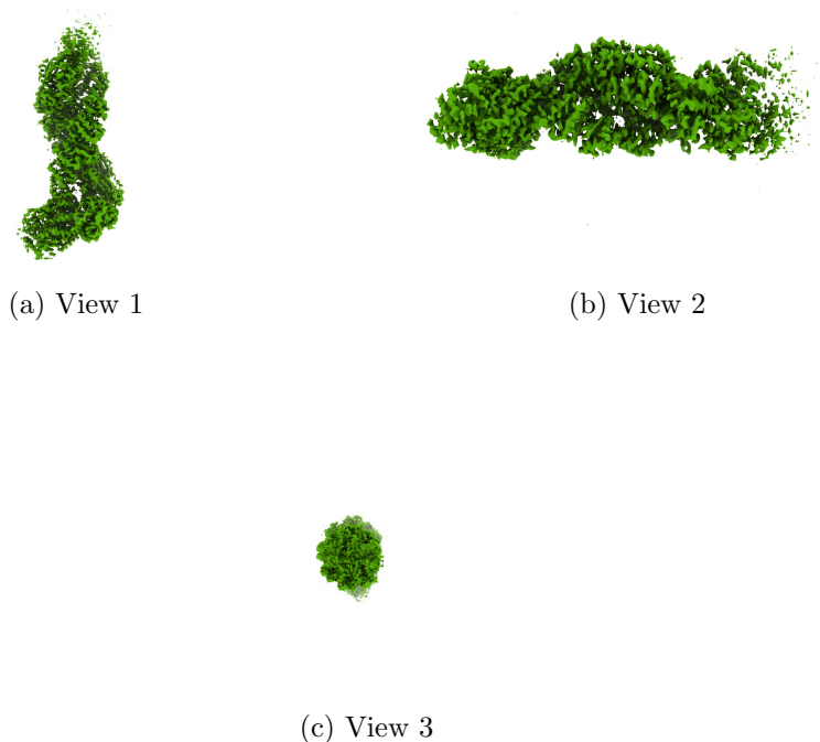
Figure 4: Isosurface at threshold=0.900000. Views generated by ChimeraX at a the following X, Y, Z angles: View 1 (0, -90, -90), View 2 (-90, 0, -90), View 3 (0, 0, 0).
