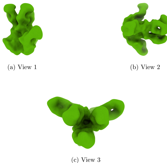
Figure 4: Isosurface at threshold=0.020200. Views generated by ChimeraX at a the following X, Y, Z angles: View 1 (0, -90, -90), View 2 (-90, 0, -90), View 3 (0, 0, 0).
