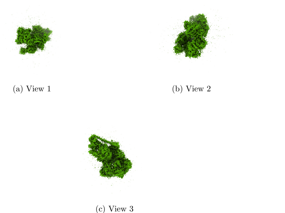
Figure 4: Isosurface at threshold=0.015000. Views generated by ChimeraX at a the following X, Y, Z angles: View 1 (0, -90, -90), View 2 (-90, 0, -90), View 3 (0, 0, 0).
