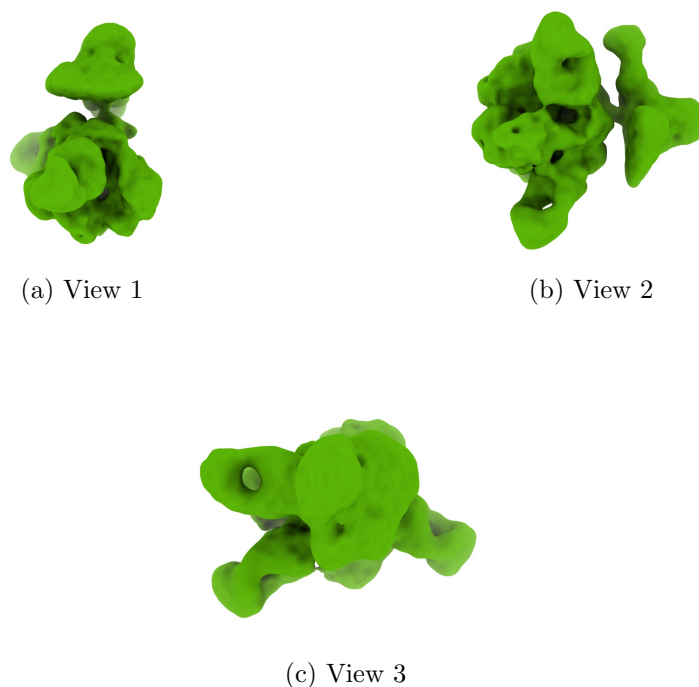
Figure 4: Isosurface at threshold=0.009000. Views generated by ChimeraX at a the following X, Y, Z angles: View 1 (0, -90, -90), View 2 (-90, 0, -90), View 3 (0, 0, 0).
