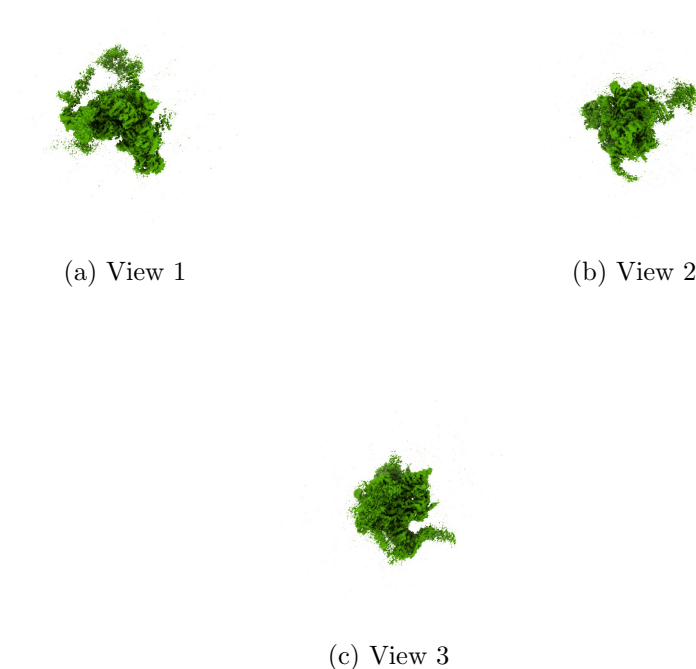
Figure 4: Isosurface at threshold=0.036000. Views generated by ChimeraX at a the following X, Y, Z angles: View 1 (0, -90, -90), View 2 (-90, 0, -90), View 3 (0, 0, 0).
