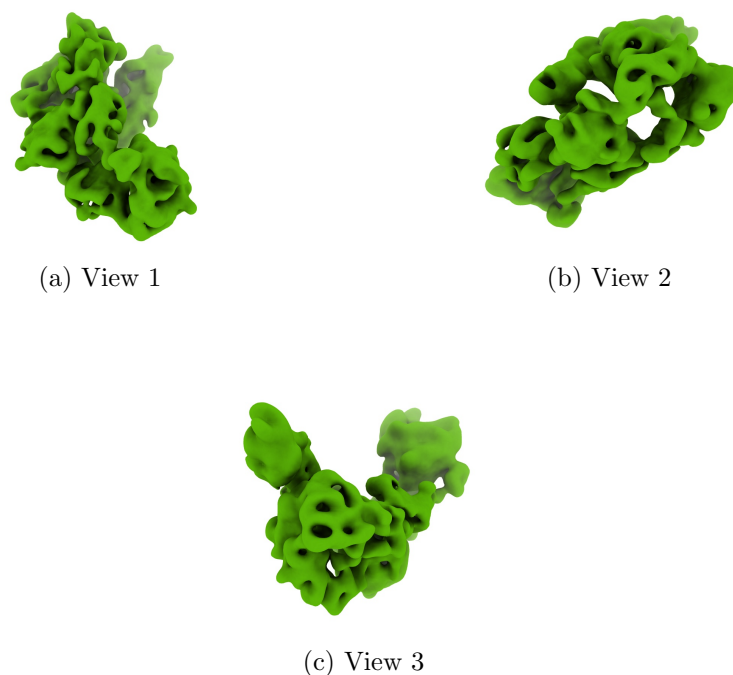
Figure 4: Isosurface at threshold=0.008210. Views generated by ChimeraX at a the following X, Y, Z angles: View 1 (0, -90, -90), View 2 (-90, 0, -90), View 3 (0, 0, 0).
