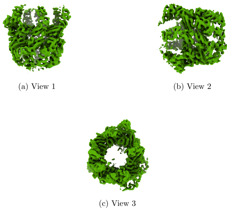
Figure 4: Isosurface at threshold=1.140000. Views generated by ChimeraX at a the following X, Y, Z angles: View 1 (0, -90, -90), View 2 (-90, 0, -90), View 3 (0, 0, 0).
