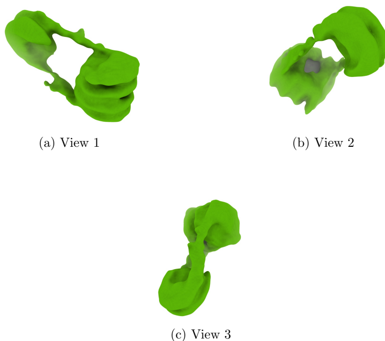
Figure 4: Isosurface at threshold=2.600000. Views generated by ChimeraX at a the following X, Y, Z angles: View 1 (0, -90, -90), View 2 (-90, 0, -90), View 3 (0, 0, 0).
