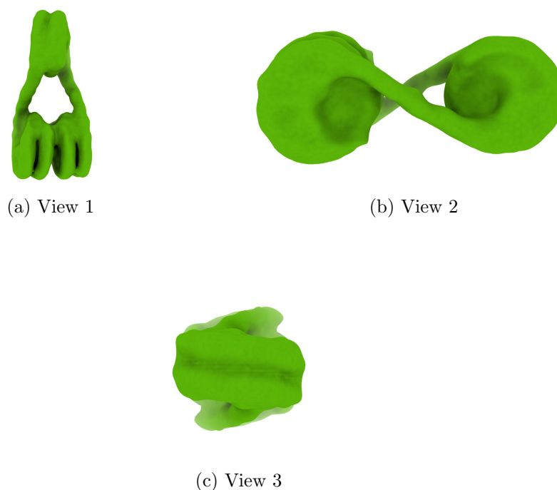
Figure 4: Isosurface at threshold=3.800000. Views generated by ChimeraX at a the following X, Y, Z angles: View 1 (0, -90, -90), View 2 (-90, 0, -90), View 3 (0, 0, 0).
