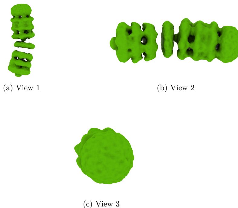
Figure 4: Isosurface at threshold=0.007700. Views generated by ChimeraX at a the following X, Y, Z angles: View 1 (0, -90, -90), View 2 (-90, 0, -90), View 3 (0, 0, 0).
