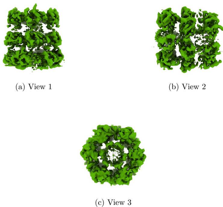
Figure 4: Isosurface at threshold=0.023600. Views generated by ChimeraX at a the following X, Y, Z angles: View 1 (0, -90, -90), View 2 (-90, 0, -90), View 3 (0, 0, 0).
