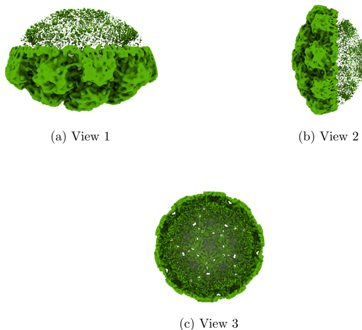
Figure 4: Isosurface at threshold=0.007730. Views generated by ChimeraX at a the following X, Y, Z angles: View 1 (0, -90, -90), View 2 (-90, 0, -90), View 3 (0, 0, 0).
