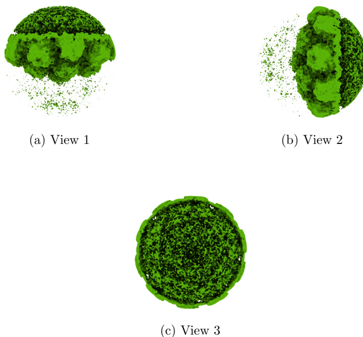
Figure 4: Isosurface at threshold=0.004490. Views generated by ChimeraX at a the following X, Y, Z angles: View 1 (0, -90, -90), View 2 (-90, 0, -90), View 3 (0, 0, 0).
