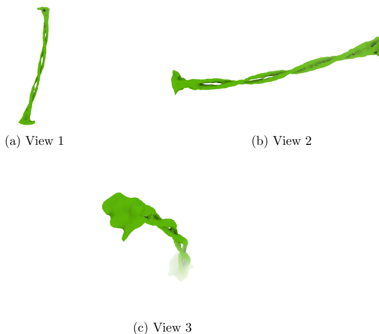
Figure 4: Isosurface at threshold=0.019000. Views generated by ChimeraX at a the following X, Y, Z angles: View 1 (0, -90, -90), View 2 (-90, 0, -90), View 3 (0, 0, 0).
