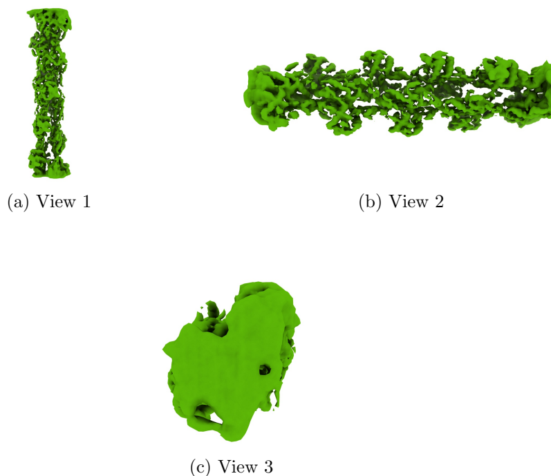
Figure 4: Isosurface at threshold=0.023000. Views generated by ChimeraX at a the following X, Y, Z angles: View 1 (0, -90, -90), View 2 (-90, 0, -90), View 3 (0, 0, 0).
