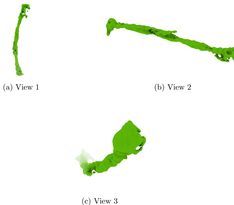
Figure 4: Isosurface at threshold=0.015600. Views generated by ChimeraX at a the following X, Y, Z angles: View 1 (0, -90, -90), View 2 (-90, 0, -90), View 3 (0, 0, 0).
