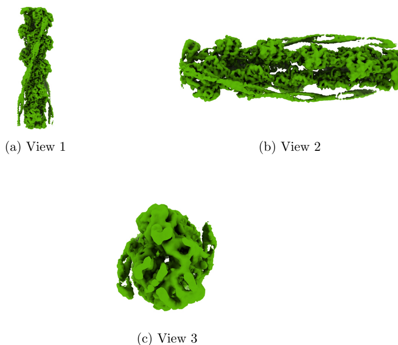
Figure 4: Isosurface at threshold=0.013500. Views generated by ChimeraX at the following X, Y, Z angles: View 1 (0, -90, -90), View 2 (-90, 0, -90), View 3 (0, 0, 0).
