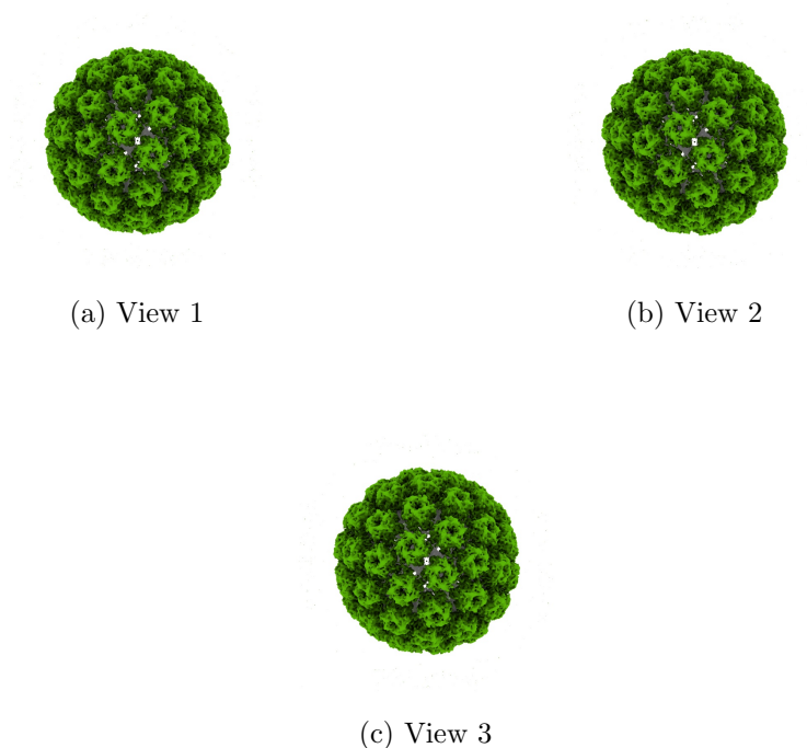
Figure 4: Isosurface at threshold=1.850000. Views generated by ChimeraX at a the following X, Y, Z angles: View 1 (0, -90, -90), View 2 (-90, 0, -90), View 3 (0, 0, 0).
