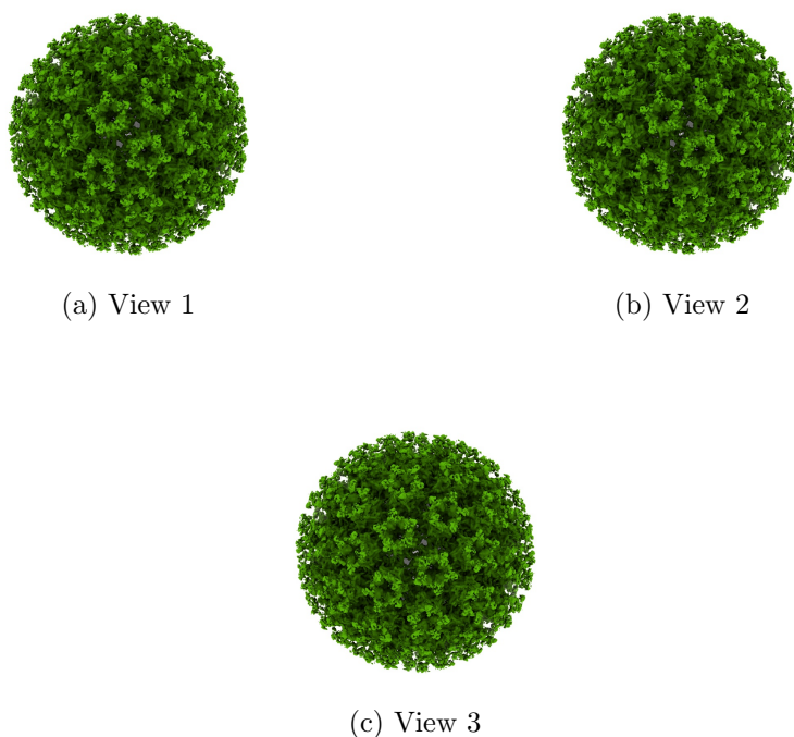
Figure 4: Isosurface at threshold=1.040000. Views generated by ChimeraX at a the following X, Y, Z angles: View 1 (0, -90, -90), View 2 (-90, 0, -90), View 3 (0, 0, 0).
