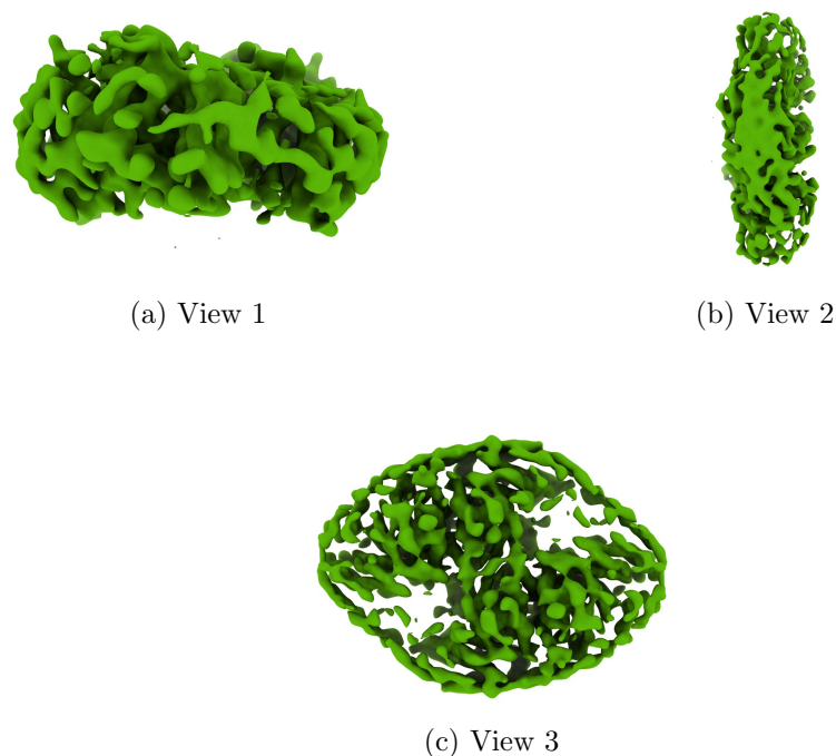
Figure 4: Isosurface at threshold=0.035000. Views generated by ChimeraX at a the following X, Y, Z angles: View 1 (0, -90, -90), View 2 (-90, 0, -90), View 3 (0, 0, 0).
